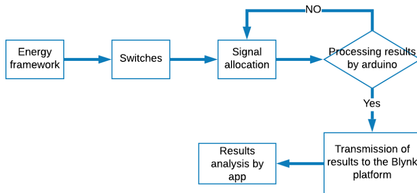
Figure 4. Application flowchart.
