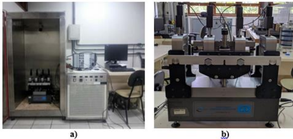
Figure 3. a) climate camera; b) 4-point test apparatus for complex module assay
