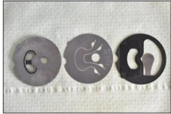
Figure 15. Valve plate, suction valve, discharge valve + gasket
