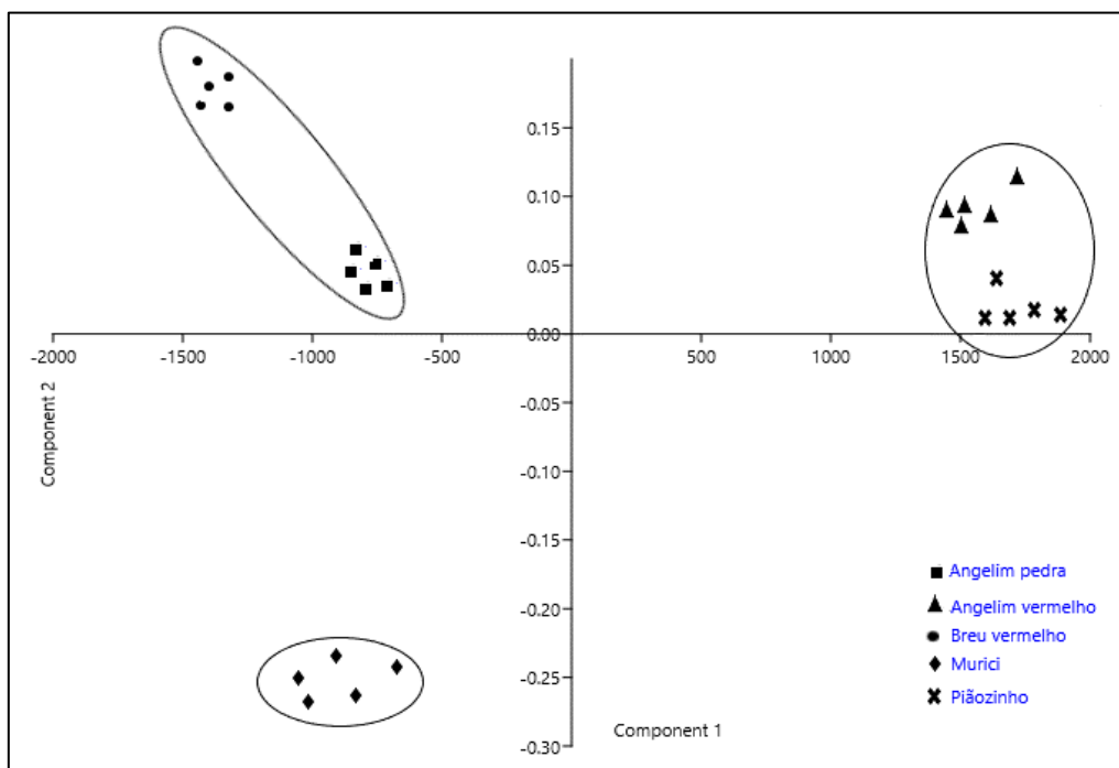
Figure 3. Analysis of the principal component of the data of the physical-mechanical properties x studied woods.
