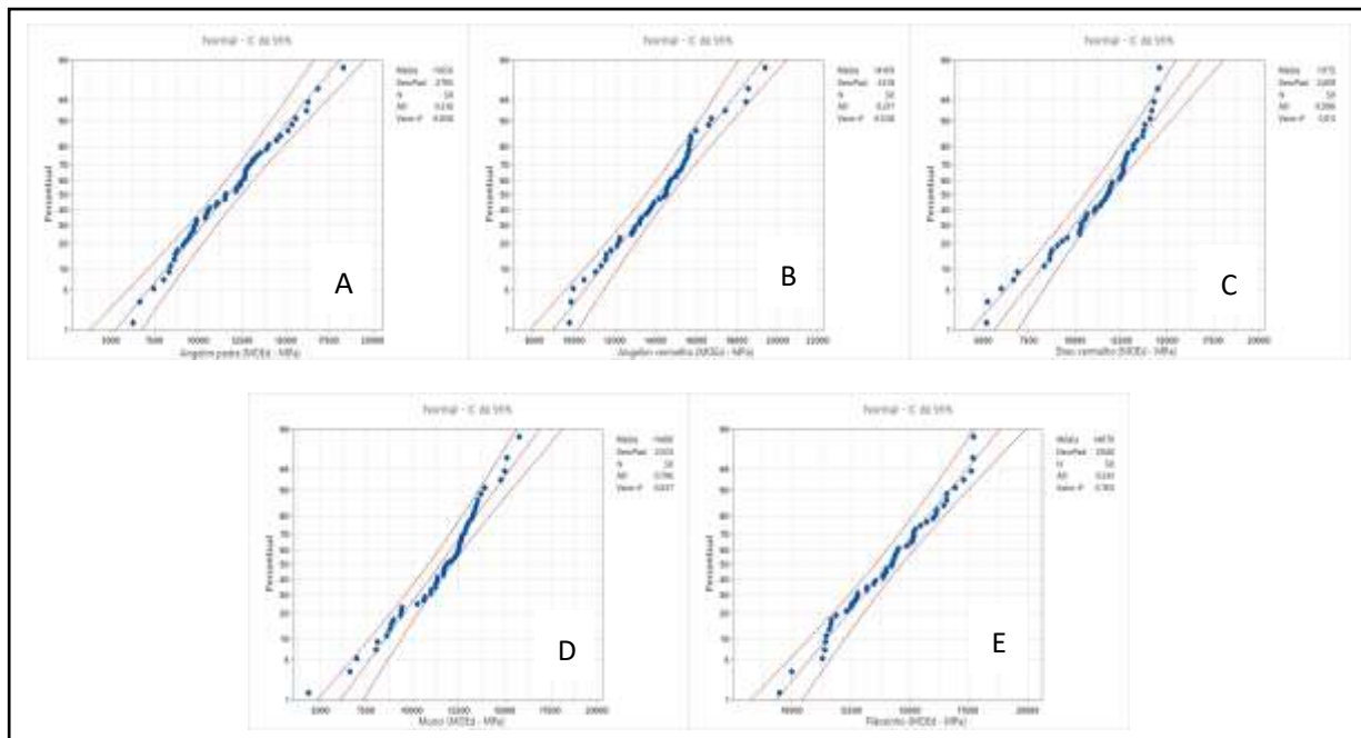
Figure 2. Probabilities of estimating the MOEd data for the studied woods: A – Angelim pedra; B – Angelim vermelho, C – Breu vermelho, D – Murici and E – Piãozinho. P-value > \alpha . P value for the Anderson-Darling (AD) normality test.
