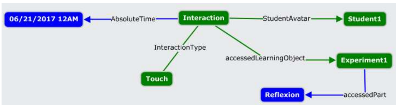
Figure 6. Instantiation of interaction with LO using the proposed Ontology
